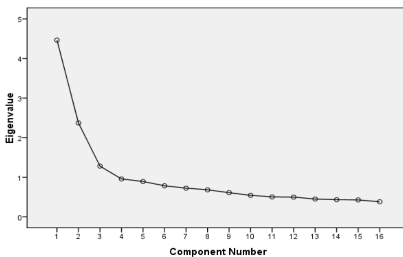
Scree Plot
